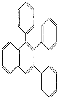
Triphenylnaphthalene
